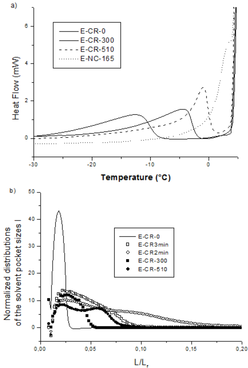
Figure 10: a) DSC-Analysis of the E-CR-0, 300, 510 and E-NC-165 swelled in cyclohexane,
