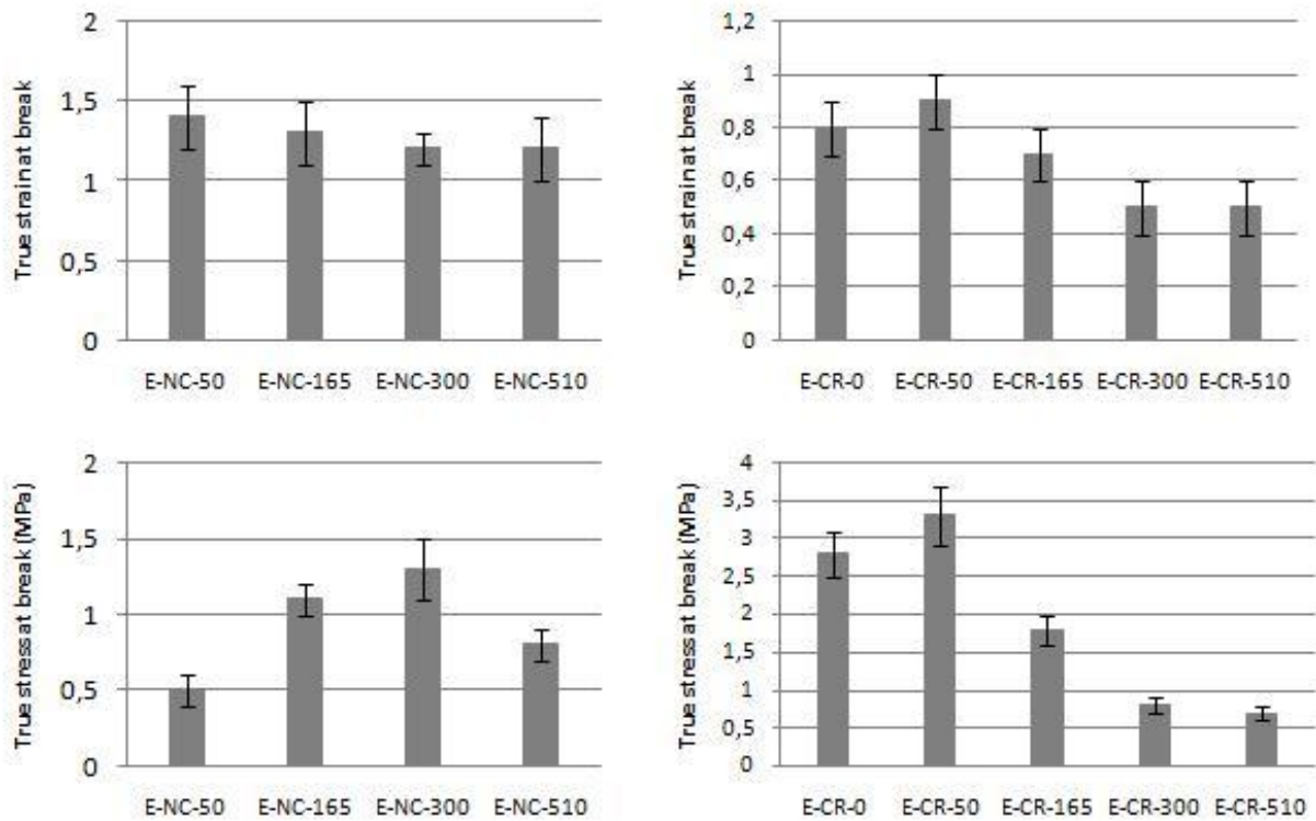
Figure 8: Average stresses and strains at break for tensile tests at 80°C of E-NC and of E-CR
