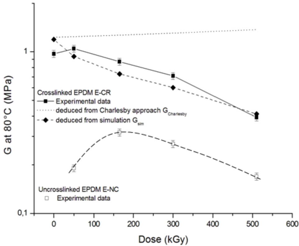
Figure 2: Evolution of the shear modulus G at 80^{\circ}\text{C} with an increasing irradiation dose for E-NC and for E-CR.
