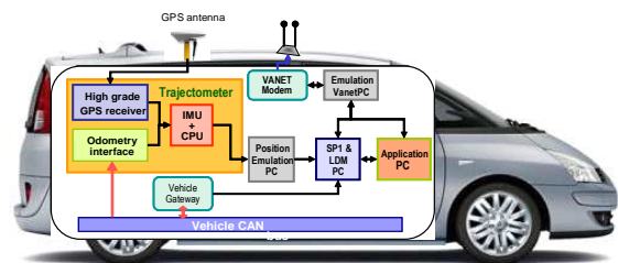
Fig. 6. Schematic representation of the implemented system
