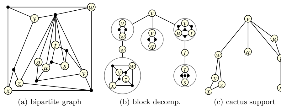
Fig. 1. Three representations of the hypergraph with hyperedges \{s, t, v\} , \{s, t, u\} , \{q, u, v\} , \{w, x, z, v\} , \{x, y, z\} , \{w, x, y\} , \{q, s, t, u, v, w, z, y\} .
