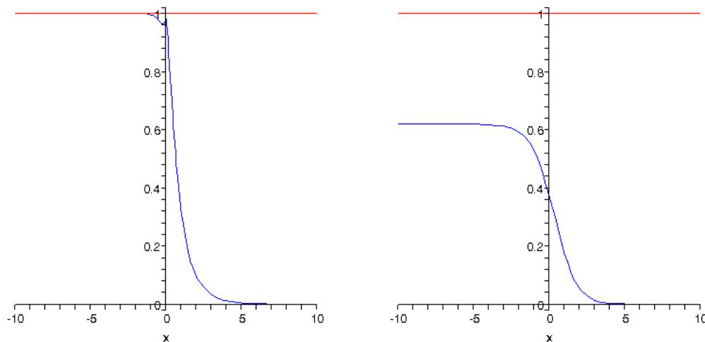
Figure 2: Behaviors of \varrho and \alpha in (\mathbb{R}^{d+1}, \ell_1) after letting w = \max\{1, \varepsilon\} . From left to right, in blue: plots of \varrho(1 + \min\{\varepsilon^2, \sqrt{\varepsilon}\}/4) and \frac{\alpha}{\varepsilon\varrho} . Both plots are versus \varepsilon on a logarithmic scale ( x = \log_{10} \varepsilon ). The red lines have equation y = 1 .
