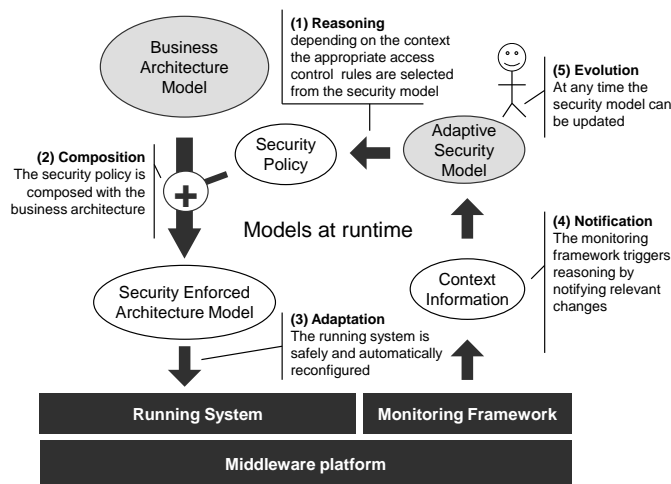
Figure 4: Overview of the proposed approach
