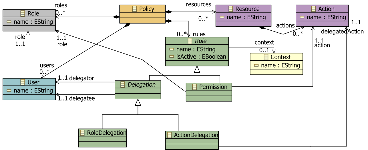
Figure 12: Access Control Metamodel
