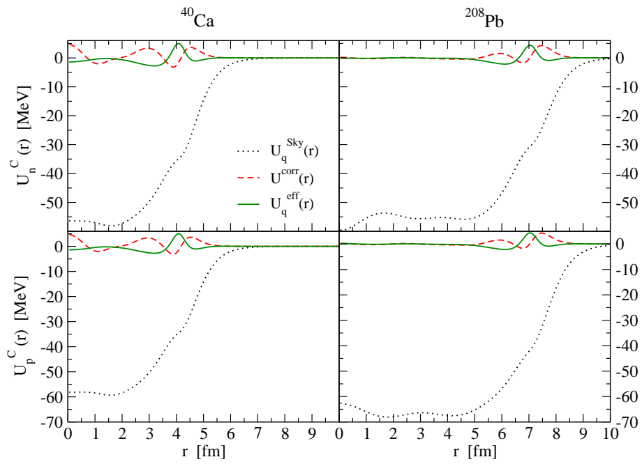
Figure 5: Central part of the neutron and proton mean field as a function of radial coordinate for ^{40}\text{Ca} and ^{208}\text{Pb} , for C_0^{\tau(\nabla\rho)^2} = -400 \text{ MeV fm}^{10} .
