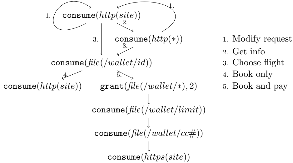
Figure 2: Example of grant/consume permissions patterns
