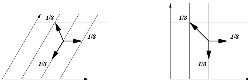
Figure 1: Random walk in the Weyl chamber of the dual of SU(3)
