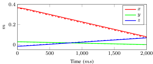
Figure 6: Reference trajectories (dash-dotted lines) and responses (solid lines) for the relative Cartesian position control in the task of pouring water
