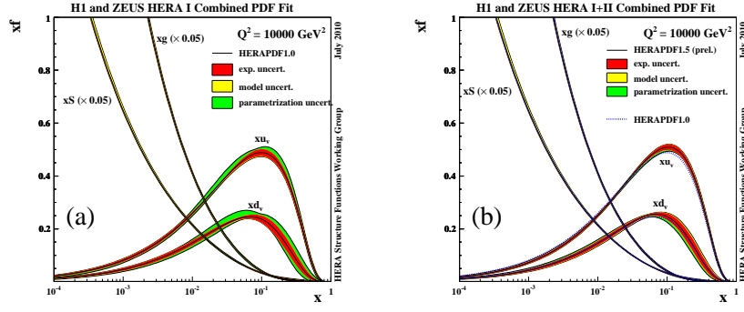
Figure 3: The parton distribution functions from HERAPDF1.0 (a) and HERAPDF1.5 (b) xu_v , xd_v , xS = 2x(\bar{U} + \bar{D}) and xg , at Q^2 = 10000 \text{ GeV}^2 .
