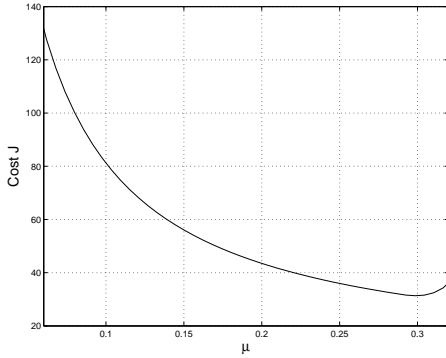
Fig. 1. Line search \mu
