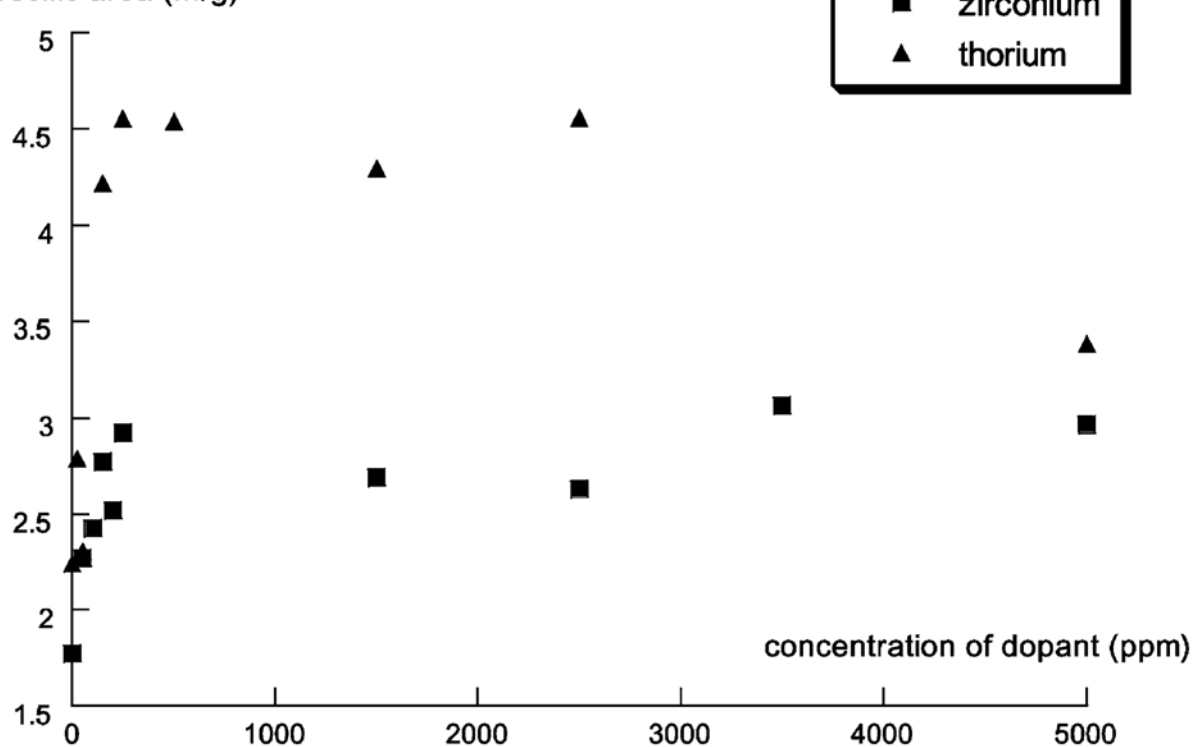
Figure 9: Specific area vs. the concentration in Zr or Th. Samples calcined under Ar+2% H_2 .
