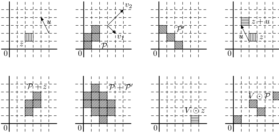
Fig. 9. Geometrical operators
