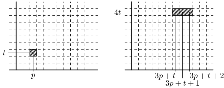
Fig. 13. Sample geometrical transform: (3, \mathbf{\Lambda}^{(3,4,1)})
