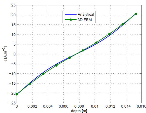
Fig.11-b. Comparison between analytical and FE computation of induced eddy-current densities along the Oz axis of the magnet, at 8 kHz
