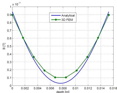
Fig. 10-b. Comparison between analytical and FE computation of magnetic flux density along the Oz axis of the magnet, at 8 kHz
