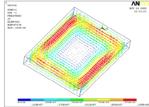
(b) Eddy-current with skin effect at frequency f= 8 kHz
