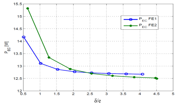
Fig. 7. Effect of mesh size on eddy-current losses in the magnet at harmonic frequency f=8 kHz. The ratio of skin depth ( \delta=5.1 mm) versus element size (e) is varying along Ox and Oz.
