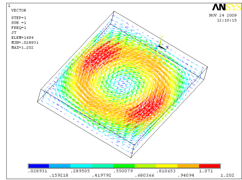
(a) Eddy-current without significant skin effect at f=1Hz
