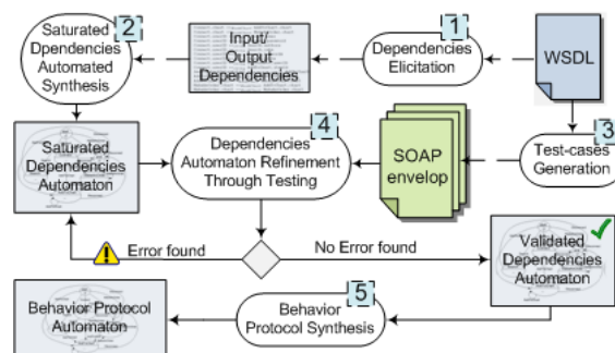
Figure 1: Overview of the Strawberry method
