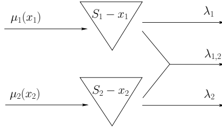
Figure 5: A system with 2 item types.
