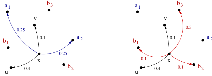
Figure 3: Redirecting the sets of transitions.
