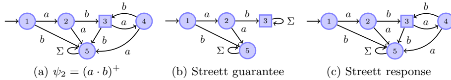
Fig. 4: DFA for \psi_2 and Streett for (E_f(\psi_2), E(\psi_2)), (R_f(\psi_2), R(\psi_2)), R = \{3\}
