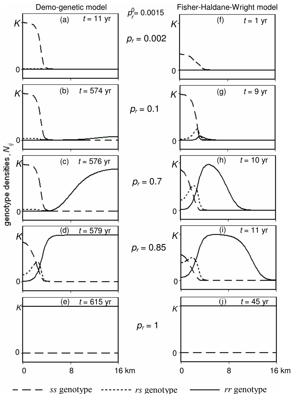
Fig. 2.15. Density distribution of ECB genotypes in a one-dimensional area 16 km long at the time (years) at which the frequency of the resistance allele p_r sequentially reaches 0.002, 0.1, 0.7, 0.85 and 1, for a 20% refuge area, in both diffusion models: demo-genetic and Fisherian.
