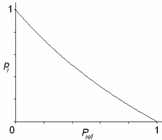
Fig. 2.8. The frequency of the Bt-resistance allele p_r as a function of the refuge fraction P_{ref} : case of the complete isolation of panmictic subpopulations in \Omega_{Bt} and \Omega_{ref} domains. Here W_{ss}^{ref} = 1 , W_{rr}^{Bt} = 0.9 , b = 1 , \mu = 0.69 .
