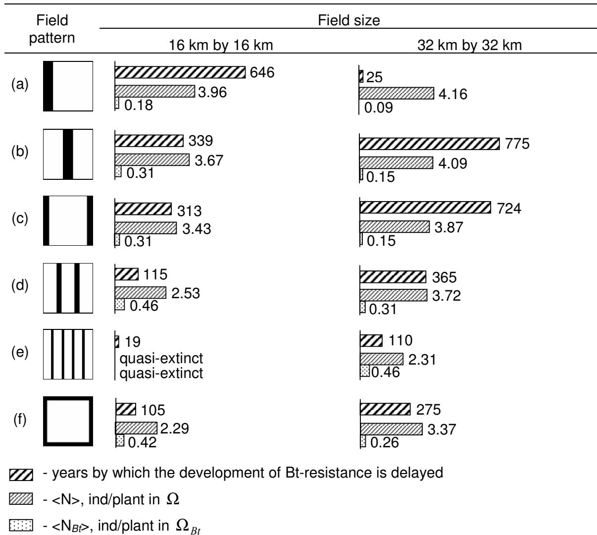
Fig. 2.16. Time T_{10} (years) required for the frequency of the resistance allele to reach 10% over the whole farming area \Omega and the levels of ECB invasion (ind/plant) of the whole maize area and the Bt area, with p_r < 0.1 (during T_{10} ), in the demo-genetic diffusion model. The refuge area is shown in black and the Bt area is shown in white. Refuges account for 20% of total area for all patterns. Pest dispersal \delta = 0.07 \text{ km}^2 \text{ yr}^{-1} .
