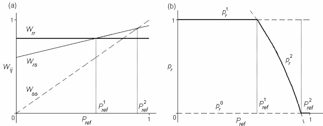
Fig. 2.7. (a) Spatially averaged genotypic fitness W_{ij} as a function of the refuge fraction P_{ref} . Dotted line corresponds to the fitness of ss genotype; thin solid line – to the fitness of rs genotype; thick solid line – to the fitness of rr genotype. (b) Frequency of the Bt-resistance allele p_r as a function of the refuge fraction P_{ref} . The stable equilibrium branches of system (2.35) are marked by thick solid line, unstable equilibrium branches are marked by dotted line. P_{ref}^1 and P_{ref}^2 are the bifurcation values of parameter P_{ref} . Given set of genetic parameters ( \sigma = 1 , c = 0.2 , h_c = 0.2 ) corresponds to the HDR strategy with high dominance level of Bt-toxin selection h_\sigma = 0.7 .
