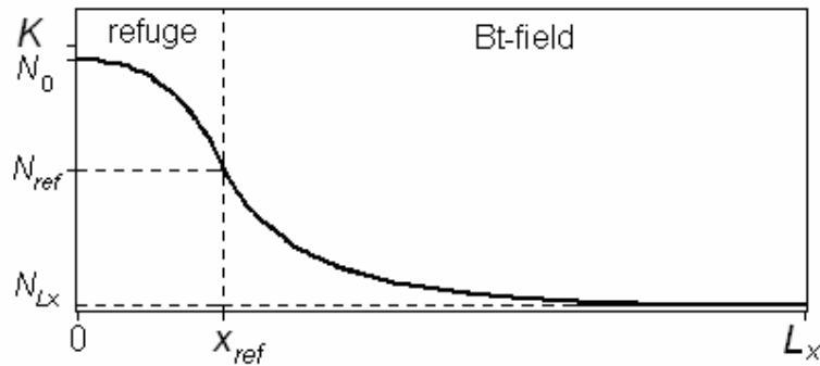
Fig. 2.11. Stationary solution of system (2.6) such that the genetic structure of the pest population consists only of individuals of ss genotype while rs and rr genotypes possessing Bt-resistance gene are absent. x_{ref} is the interface point between Bt-field (80%) and refuge (20%).
