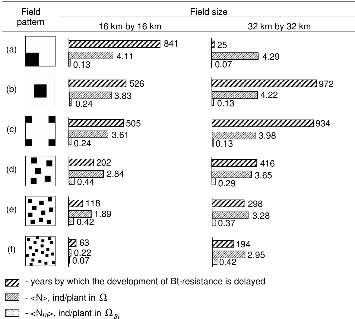
Fig. 2.17. Time T_{10} (years) required for the frequency of the resistance allele to reach 10% over the whole farming area \Omega and the levels of ECB invasion (ind/plant) of the whole maize area and the Bt area, with p_r < 0.1 (during T_{10} ), in the demo-genetic diffusion model. The refuge area is shown in black and the Bt area is shown in white. Refuges account for 20% of total area for all patterns. Pest dispersal \delta = 0.07 \text{ km}^2 \text{ yr}^{-1} .
