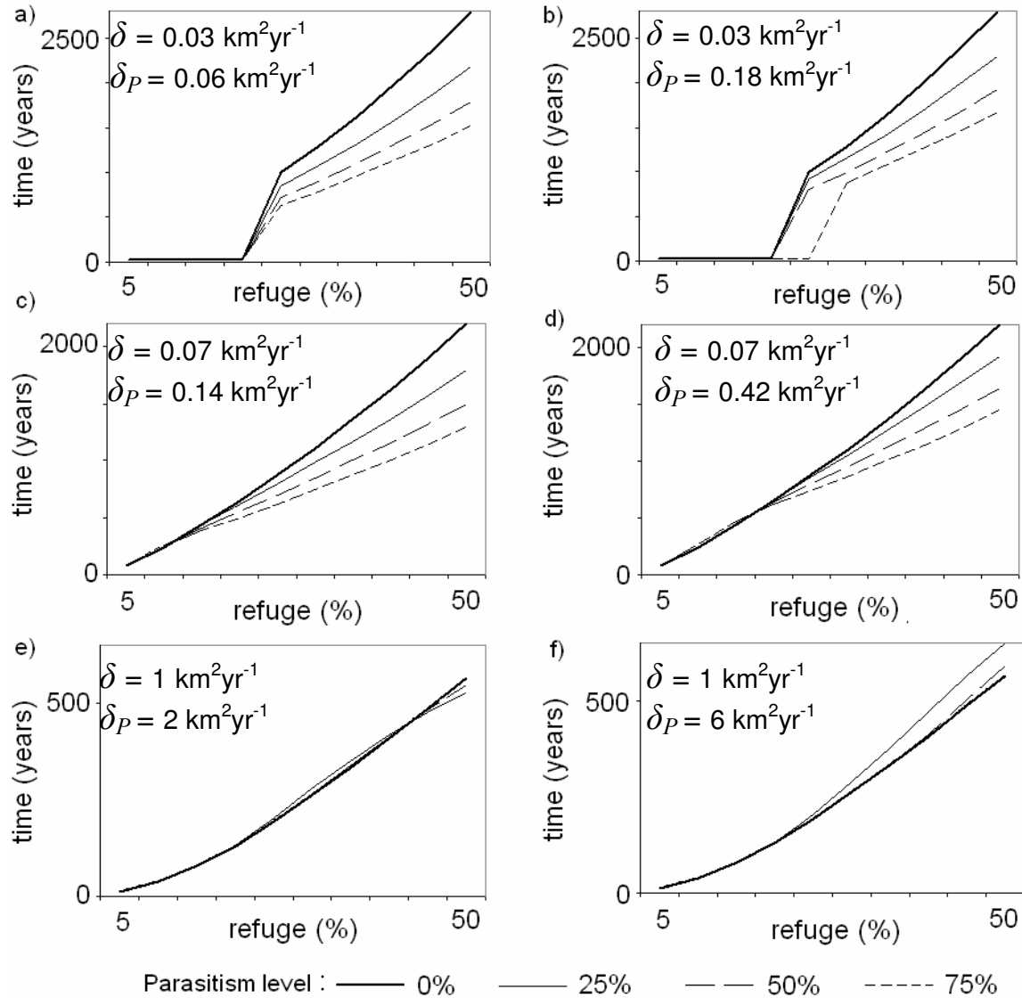
Fig. 3.1. Time T_{10} (years) required for the frequency of the resistance allele to reach 10% over the entire farming area \Omega in the demo-genetic model (3.2) with different dispersals of pest \delta and its parasitoid \delta_p .
