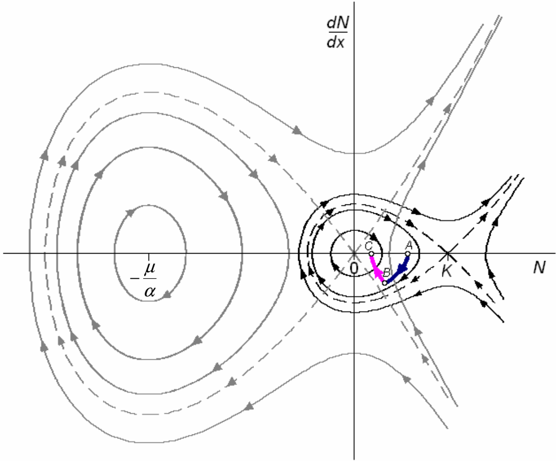
Fig. 2.12. Phase portrait of system (2.41). Phase trajectories of system are marked with black lines in the refuge \Omega_{ref} and with grey lines in the Bt-field \Omega_{Bt} . Separatrices are marked with dotted lines. Arc AB corresponds to the section of the closed phase trajectory which is generated by system within the refuge. Arc BC corresponds to the section of the non-closed phase trajectory of hyperbolic type, which is generated by system within the Bt-field.
