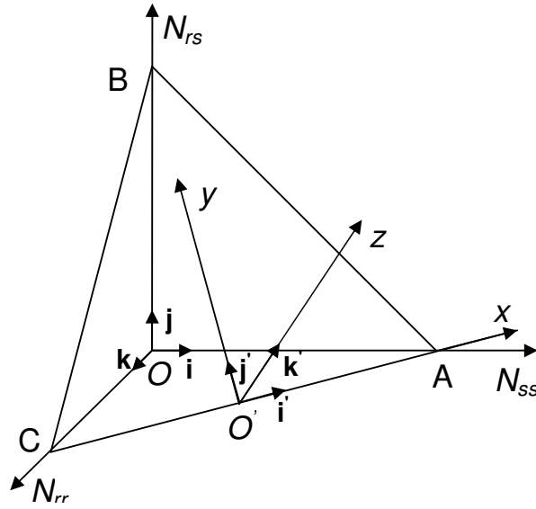
Fig. 2.1. Transition from the old basis (\mathbf{i}, \mathbf{j}, \mathbf{k}) to the new one (\mathbf{i}', \mathbf{j}', \mathbf{k}') . N_{ss} , N_{rs} , N_{rr} are the densities of corresponding pest genotypes.
