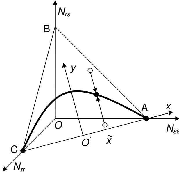
Fig. 2.2. Equilibrium family of system (2.11) is a parabola (thick solid line) on plane ABC. N_{ss} , N_{rs} , N_{rr} are the densities of corresponding pest genotypes.
