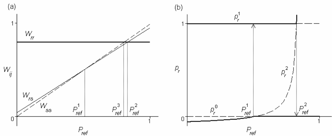
Fig. 2.5. (a) Spatially averaged genotypic fitness W_{ij} as a function of the refuge fraction P_{ref} . Dotted line corresponds to the fitness of ss genotype; thin solid line – to the fitness of rs genotype; thick solid line – to the fitness of rr genotype. (b) Frequency of the Bt-resistance allele p_r as a function of the refuge fraction P_{ref} . The stable equilibrium branches of system (2.35) are marked by thick solid line, unstable equilibrium branches are marked by dotted line. P_{ref}^1 and P_{ref}^2 are the bifurcation values of parameter P_{ref} . Given set of genetic parameters ( \sigma = 1 , c = 0.2 , h_c = 0.2 ) corresponds to the HDR strategy with low dominance level of Bt-toxin selection h_\sigma = 0.05 .
