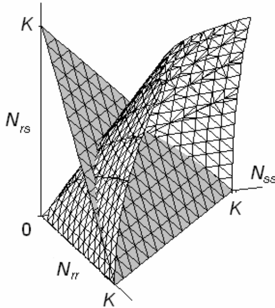
Fig. 2.3. The Hardy-Weinberg equilibrium u_{ss}u_{rr} = \frac{u_{rs}^2}{4} in three-dimensional space of phase variables (N_{ss}, N_{rs}, N_{rr}) defines the surface of cone (marked in white), where u_{ij} = \frac{N_{ij}}{N} , N = N_{ss} + N_{rs} + N_{rr} = K (the grey plane), N_{ss} , N_{rs} , N_{rr} are the densities of corresponding genotypes.
