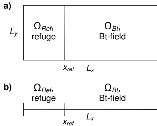
Fig. 2.9. (a) Border single-strip refuge pattern for the rectangular habitat \Omega . (b) Its 1D simplification in the absence of the density fluxes of the pest genotypes along the side L_y .
