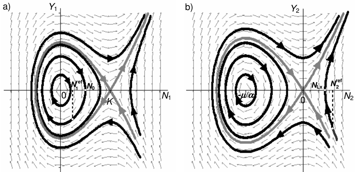
Fig. 2.10. Phase portraits of the stationary system for the population consisting solely of insects of ss genotype dwelling in the refuge (a) and in the Bt-field (b). Some phase trajectories are marked with thick lines; separatrices are marked with grey thick lines. Arrows define the directional field of the system.
