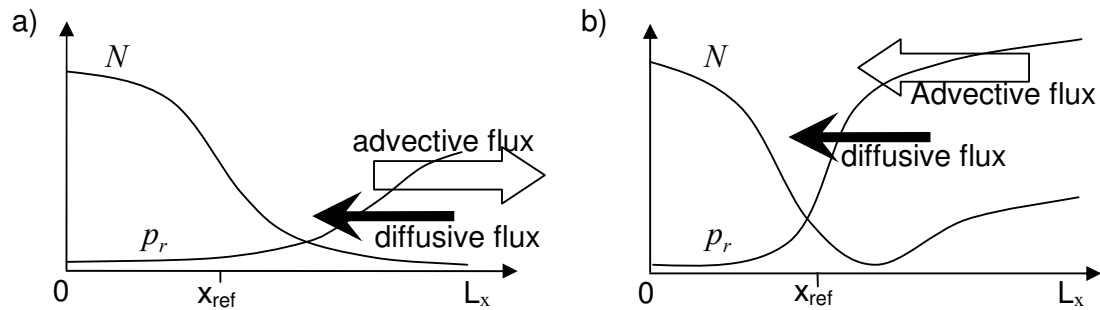
Fig. 2.19. Scheme of spatial distribution of frequency p_r and total density N in the demo-genetic model (2.32) in 1D habitat when (a) the density of resistant insects in the Bt-field is very low ( \approx 0 ) and (b) the density of resistant insects in the Bt-field increased due to the spatial dispersal of the Bt-resistance gene in the pest population.
