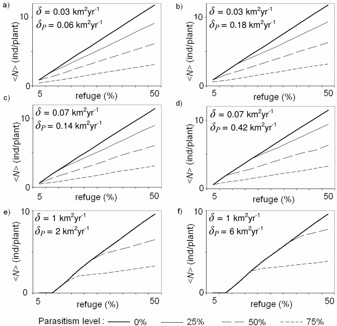
Fig. 3.2. Spatially averaged pest density, maintained in the ECB population throughout the entire habitat \Omega as long as p_r < 10\% in the demo-genetic model (3.2) with different dispersals of pest \delta and its parasitoid \delta_P .
