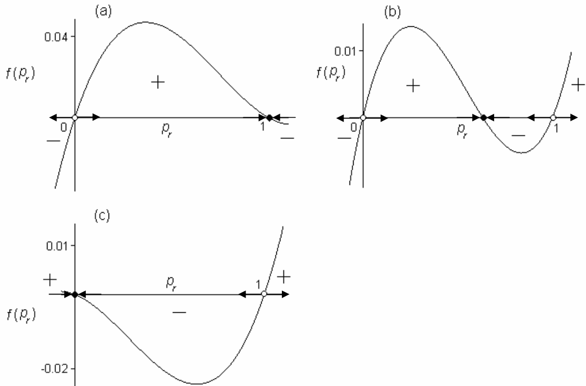
Fig. 2.6. Right-hand part of equation (2.35) f(p_r) as a function of the frequency of the Bt-resistance allele, p_r , for various refuge fractions P_{ref} : (a) P_{ref} < P_{ref}^1 ; (b) P_{ref} \in (P_{ref}^1, P_{ref}^2) ; (c) P_{ref} > P_{ref}^2 . The stable equilibria of system (2.35) are marked with black circles and the unstable equilibria are marked with white circles. Given set of genetic parameters ( \sigma=1 , c=0.2 , h_c=0.2 ) corresponds to the HDR strategy with high dominance level of the Bt-toxin selection h_\sigma=0.7 .
