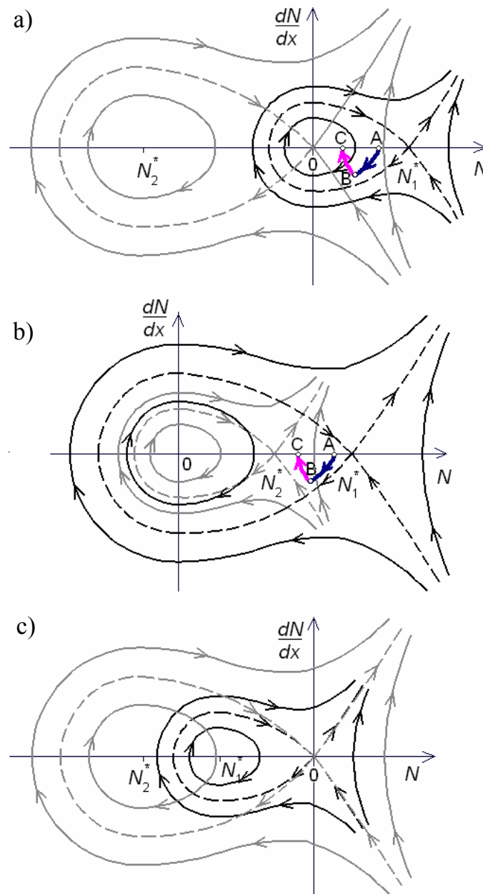
Fig. 2.13. Phase portraits of system (2.41) in the case of W_{ss}^{Bt} < W_{ss}^{ref} . Here N_1^* = (W_{ss}^{ref} b - \mu)/\alpha , N_2^* = (W_{ss}^{Bt} b - \mu)/\alpha . (a) W_{ss}^{ref} > \mu/b , W_{ss}^{Bt} < \mu/b ; (b) W_{ss}^{ref} > \mu/b , W_{ss}^{Bt} > \mu/b ; (c) W_{ss}^{Bt} < W_{ss}^{ref} < \mu/b . Phase trajectories of system are marked with black lines in the refuge \Omega_{ref} and with grey lines in the Bt-field \Omega_{Bt} . Separatrices are marked with dotted lines. Arc AB corresponds to the section of the closed phase trajectory of the system within the refuge. Arc BC corresponds to the section of the non-closed phase trajectory of hyperbolic type that is generated by system within the Bt-field. Point A corresponds to the left boundary condition of problem (2.41), point C – to the right-hand one. Point B is the point of sewing together the solutions in the refuge and in the Bt-field.
