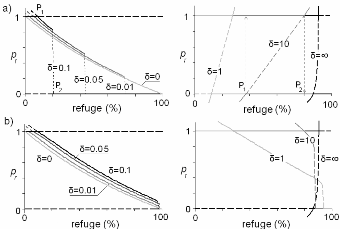
Fig. 2.14. Frequency of the Bt-resistance allele p_r as a function of refuge percentage for (a) the demo-genetic model (2.6) and (b) the Fisher-Haldane-Wright model. The branches of stable equilibria are marked with solid lines. The branches of unstable equilibria are marked with dotted lines. A given set of genetic parameters corresponds to the HDR strategy: \sigma = 1 , c = 0.1 , h_\sigma = 0.14 , h_c = 0.2 .
