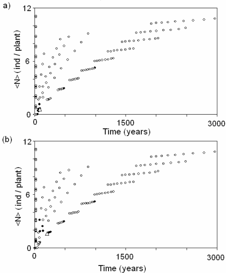
Fig. 2.18. A Pareto diagram for two criteria: time T_{10} (years) required for the frequency of the resistance allele to reach 10% over the whole farming area \Omega and the levels of ECB invasion (ind/plant) of the whole maize area, with p_r < 0.1 (during T_{10} ). (a) \rho = 5.75\% ; (b) \rho = 0 . The optimal refuge sizes \Omega_{ref} which provide the maximum of profit \Pi with different fixed habitat sizes \Omega are marked with black circles. The optimal parameters (\Omega, \Omega_{ref}) with respect to three criteria ( T_{10} , \langle N \rangle , \Pi ) are marked with triangles.
