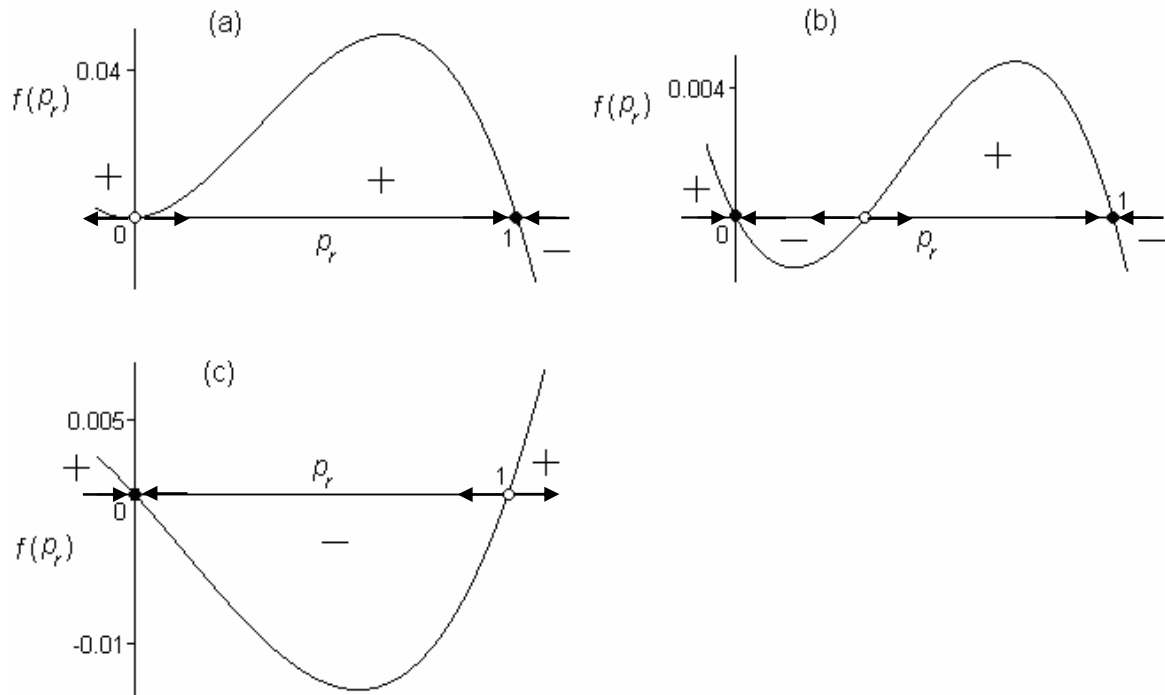
Fig. 2.4. Right-hand part of equation (2.35) f(p_r) as a function of the frequency of the Bt-resistance allele, p_r , for various refuge fractions P_{ref} : (a) P_{ref} = P_{ref}^1 ; (b) P_{ref} \in (P_{ref}^1, P_{ref}^2) ; (c) P_{ref} > P_{ref}^2 . The stable equilibria of system (2.35) are marked with black circles and the unstable equilibria are marked with white circles. The given set of genetic parameters ( \sigma = 1 , c = 0.2 , h_c = 0.2 ) corresponds to the HDR strategy with low dominance level of the Bt-toxin selection h_\sigma = 0.05 .
