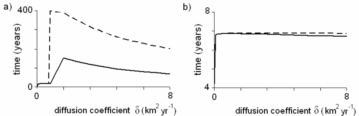
Fig. 3.3 Time T_{10} (years) required for the frequency of the resistance allele to reach 10% as a function of pest mobility \delta predicted by (A): the bi-trophic demo-genetic model “resource – pest” (3.5) and (B) the diffusional model based on the Fisherian equations (model (3.5) without the advective term in equation for p_r ) with 10% (solid line) and 20% (dashed line) single-strip refuge.
