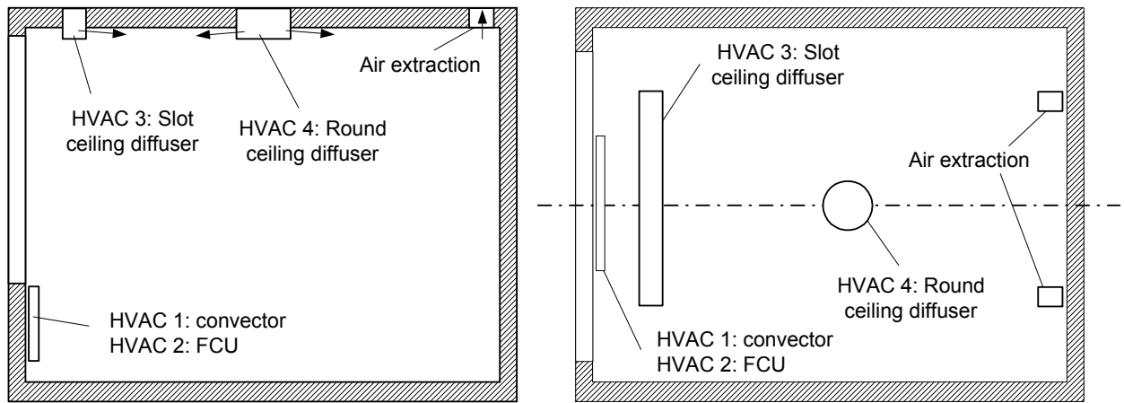
Figure V - 2: HVAC systems used for the study (left: vertical cross-section; right: plan)
