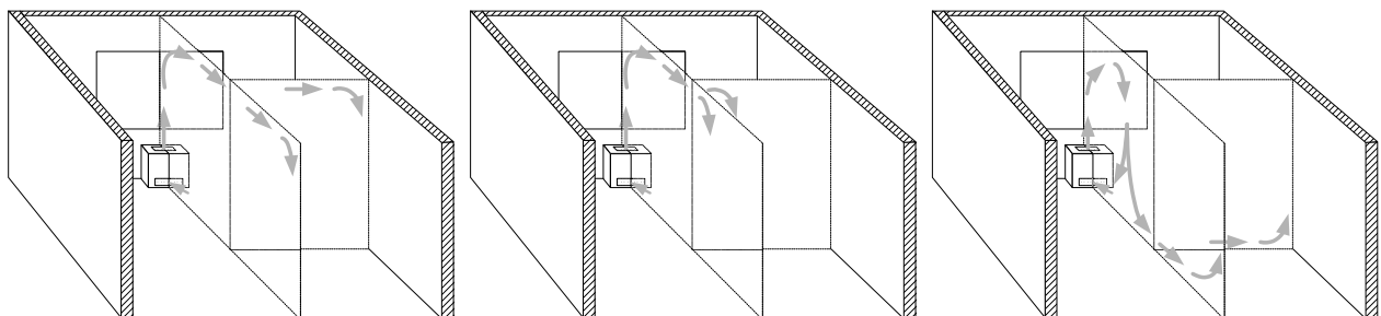
Figure II - 3: Airflow pattern: type 1 – high positive buoyancy forces
