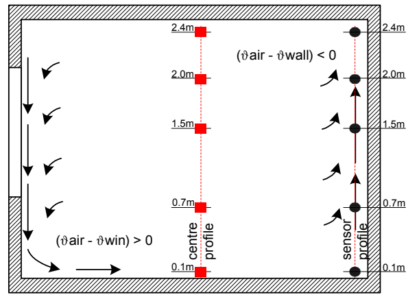
Figure II - 30: Qualitative airflow pattern in the winter case - EREDIS
