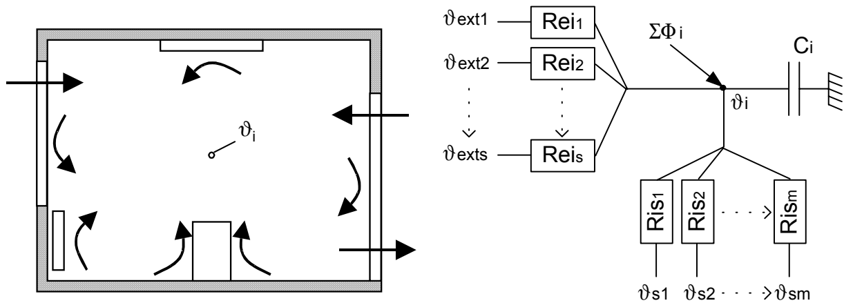
Figure III - 6: Heat exchanges in the well mixed model (left) and electrical representation (right)
