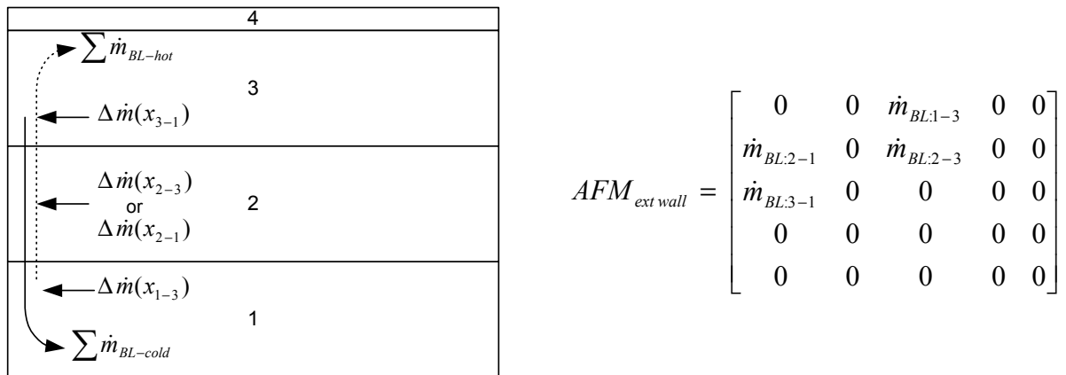
Figure IV - 22: Air flow due to the boundary layer at the external surfaces
