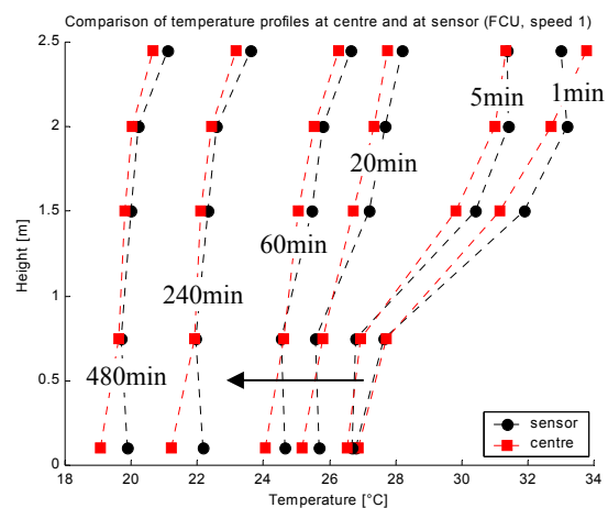
Figure II - 54: Evolution of centre and sensor temperature profile (test OFF → ON) - EREDIS
