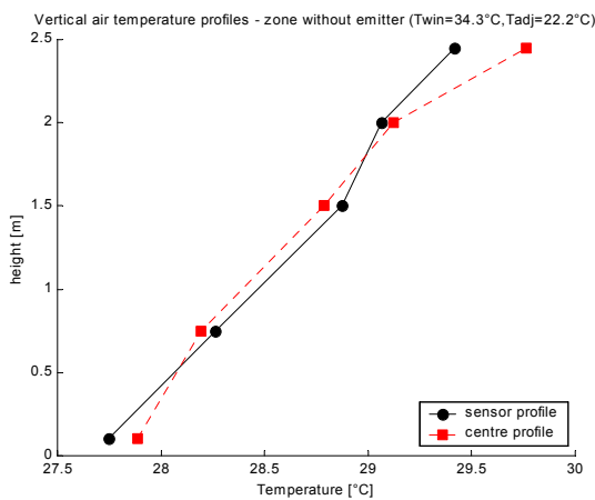
Figure II - 31: Temperature profiles at centre and sensor position for the case without cooling (summer case) - EREDIS
