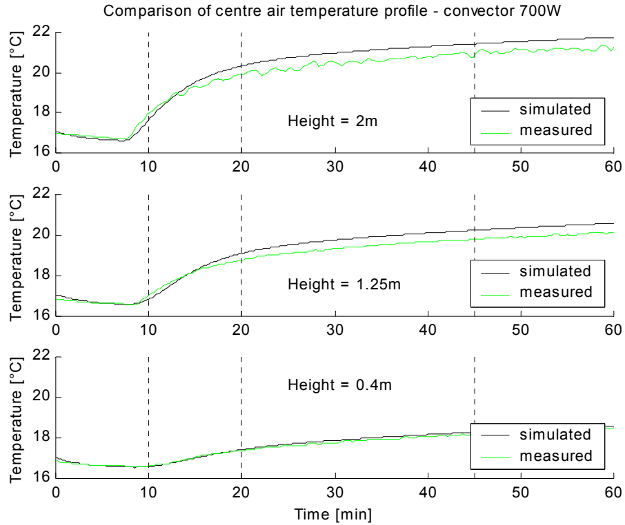
Figure IV - 37: Validation of the room model for the electric convector - centre temperature - 700W
