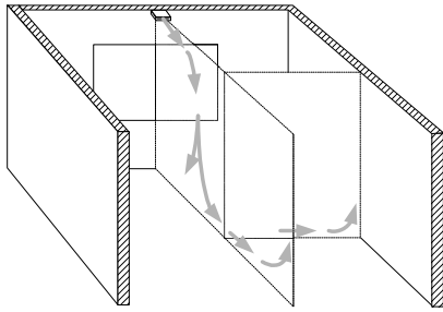
Figure II - 6: Airflow pattern: type 2 – high positive buoyancy forces
