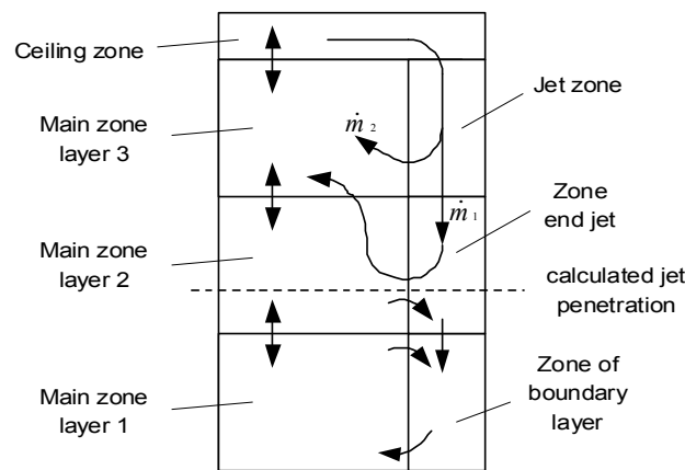
Figure IV - 14: Air flow in the sub-volumes at the internal walls in the case of negatively buoyant flow
