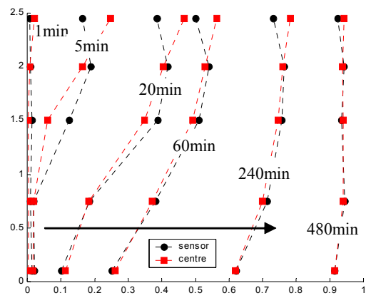
Figure II - 52: Evolution of centre - sensor relative temperature profile (test OFF → ON) - EREDIS
