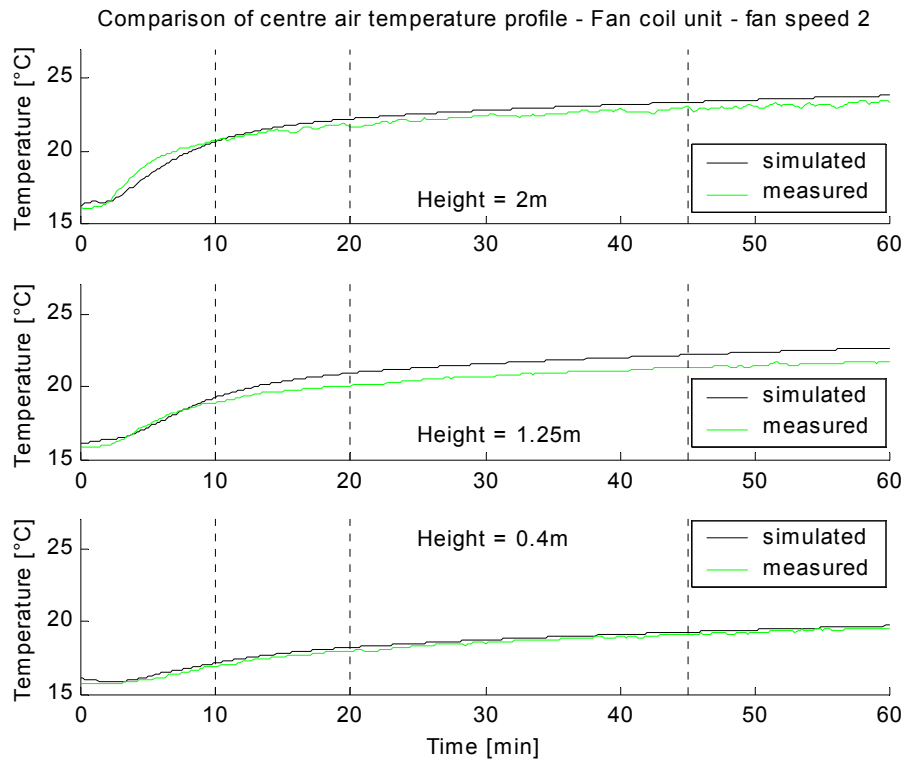
Figure IV - 43: Validation of the room model for the fan coil unit - centre temperature - fan speed 2
