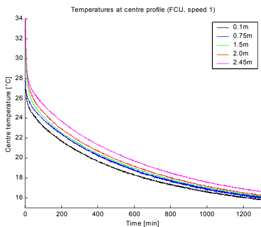
Figure II - 53: Evolution of air temperatures at centre profile (test ON → OFF) - EREDIS
