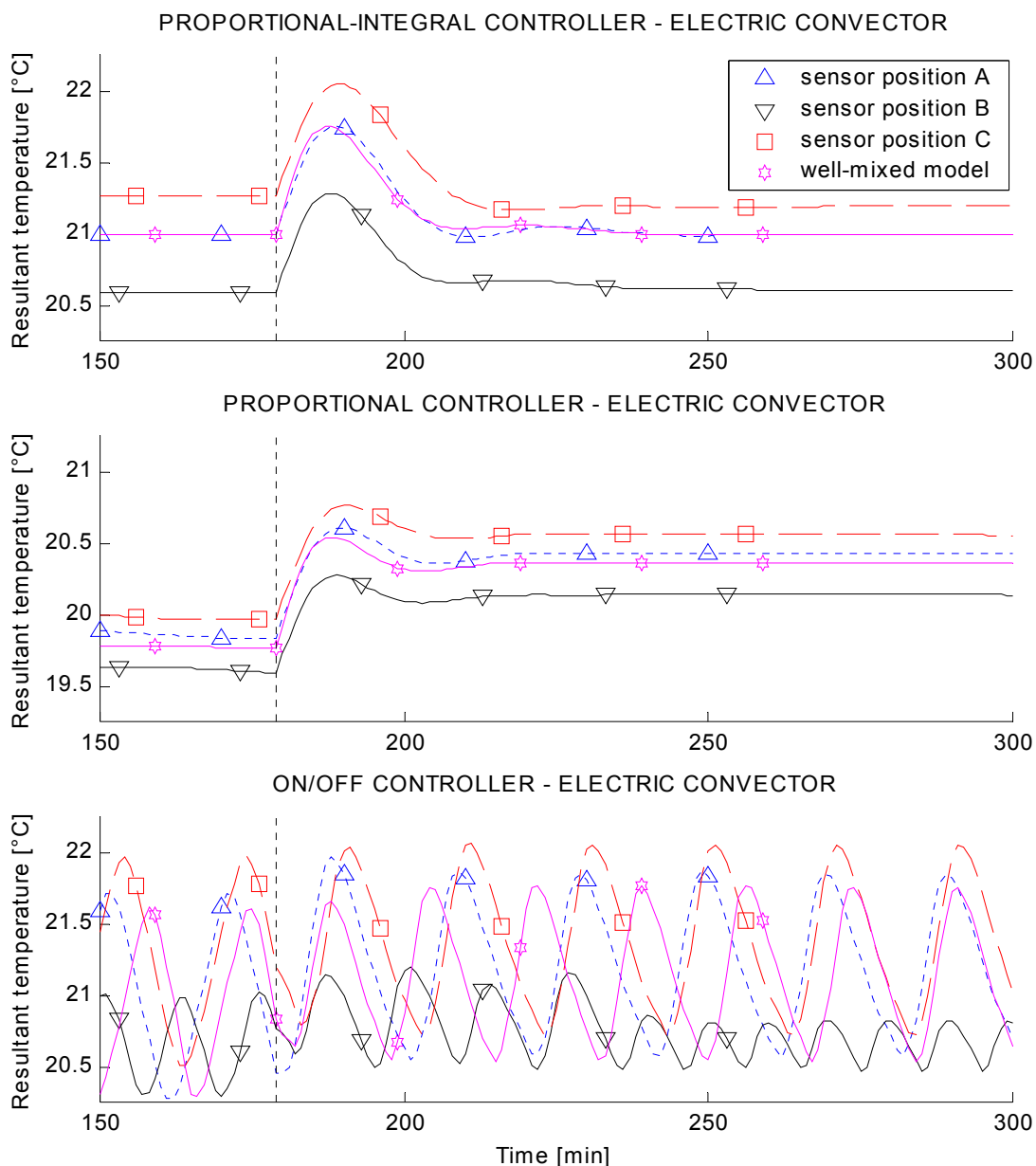
Figure V - 6: Resultant temperature - electric convector
