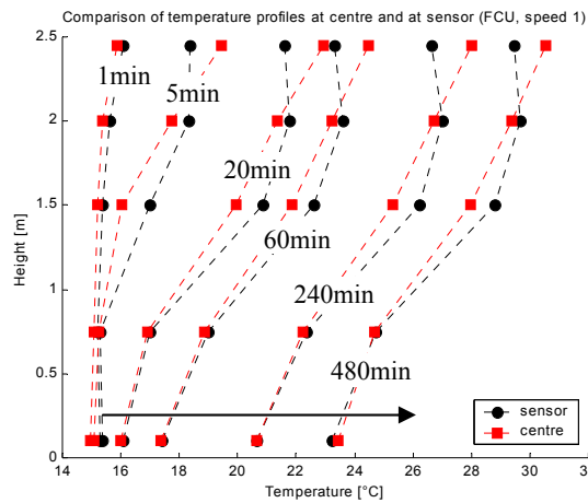
Figure II - 50: Evolution of centre and sensor temperature profile (test OFF → ON) - EREDIS
