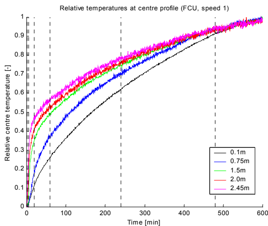
Figure II - 51: Evolution of relative temperature at centre profile (test OFF → ON) - EREDIS
