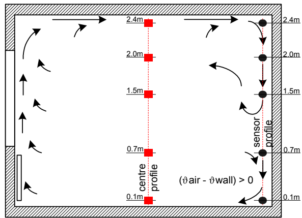
Figure II - 34: Qualitative airflow pattern with a convector – favourable boundary layer
