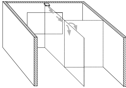
Figure II - 7: Airflow pattern: type 2 – low buoyancy forces
