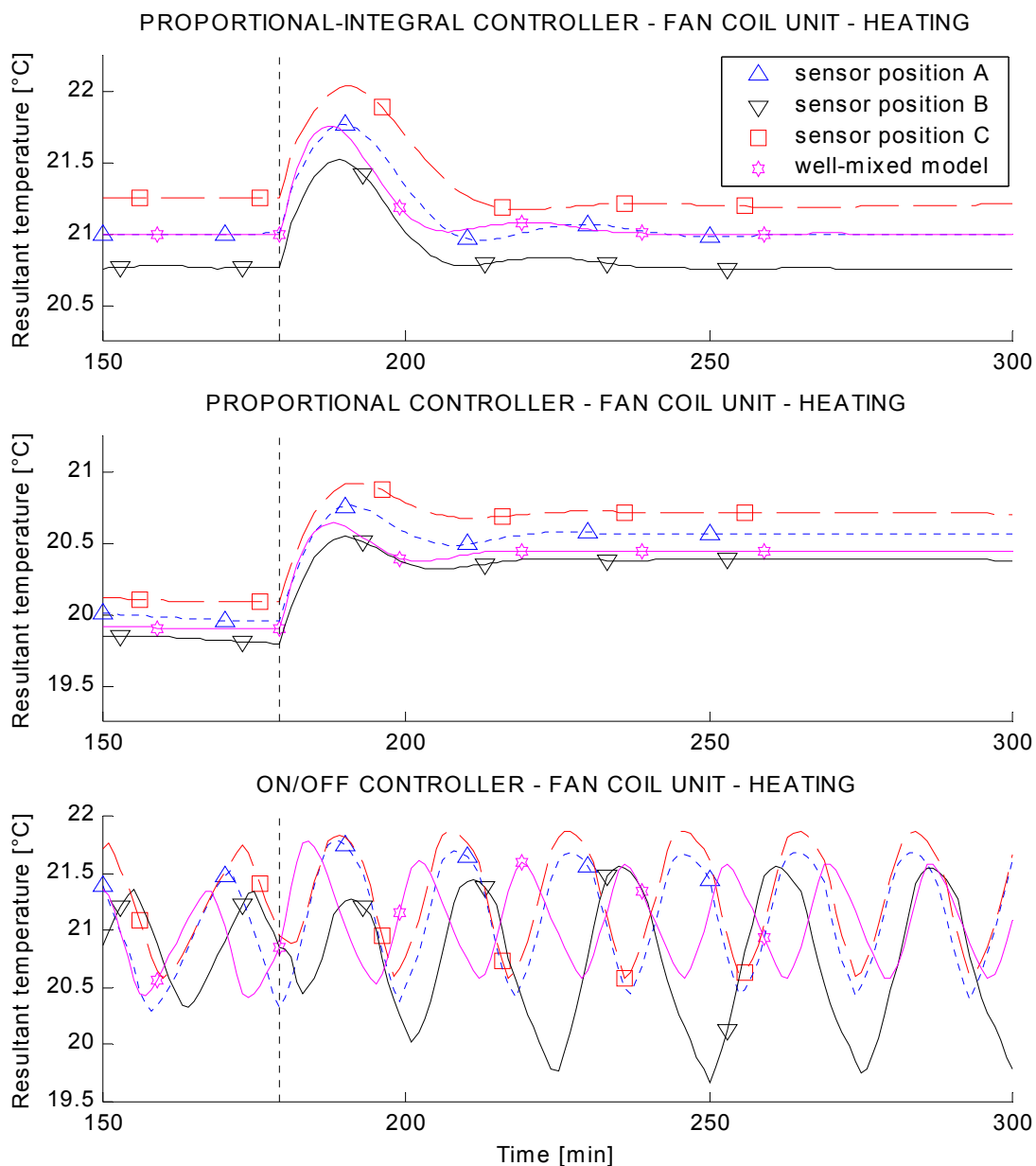
Figure V - 9: Resultant temperature - fan coil unit - heating
