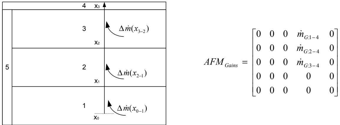
Figure IV - 21: Air flow due to plumes from internal heat gains
