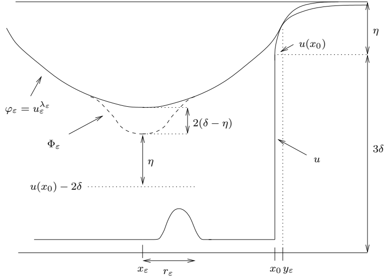
Figure 1: One possible situation of the chosen test functions.
