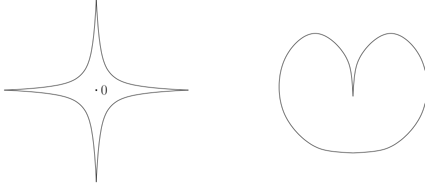
FIGURE 1. A set which is star-shaped with respect to 0 but does not satisfy (I2) and a set whose boundary is not locally Lipschitz continuous and which satisfies (I2).
