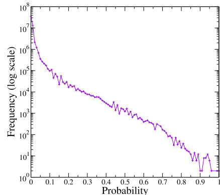
Figure 16: Distribution of probabilities in the bootstrap probabilistic graph.
