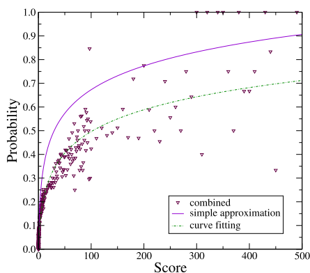
Figure 15: Mapping scores to probabilities, for generating the bootstrap probabilistic graph.
