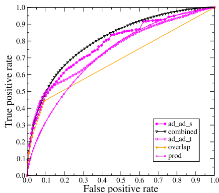
Figure 14: ROC curves for the best feature from each category and the best combined feature.
