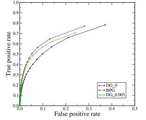
Figure 19: ROC curves for the rooted_pagerank feature.
