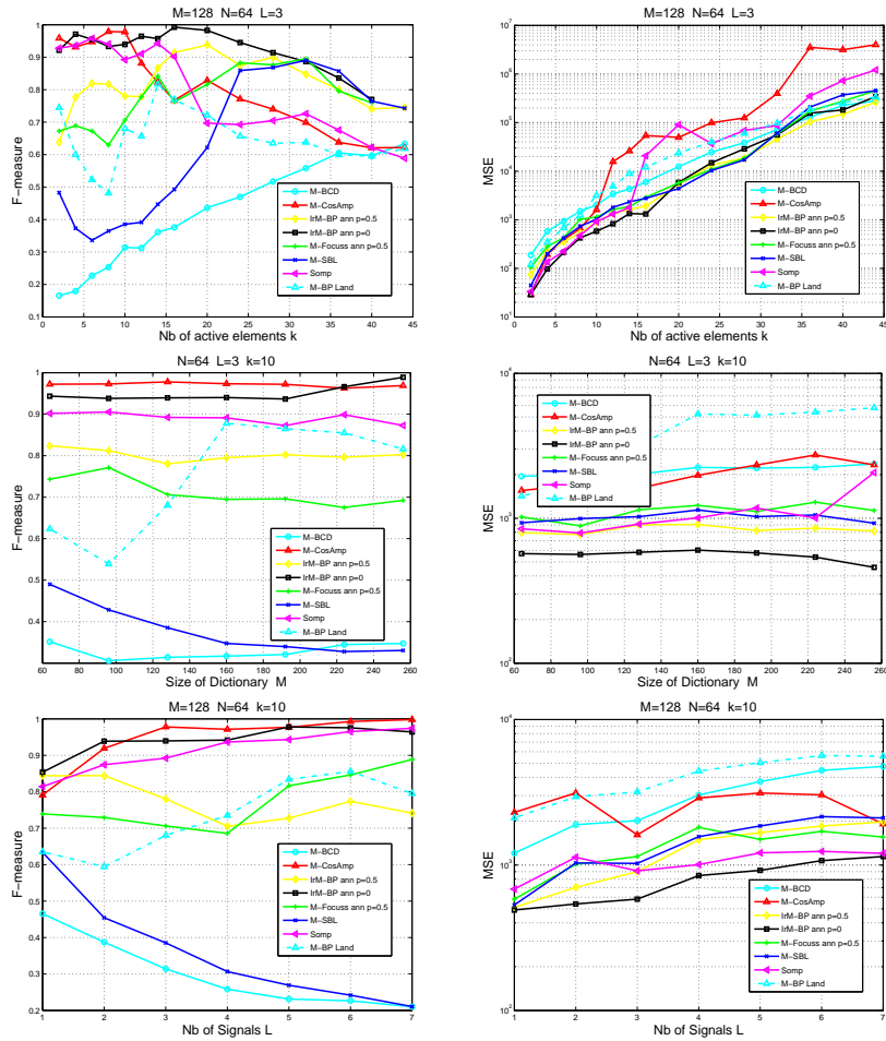
Figure 3: Results comparing performances of different simultaneous sparse algorithms. We have varied (top) the number k of active elements in the dictionary. (middle) the dictionary size M and (bottom) the number of signal to approximate L . On the left columns are given the F-measure of all methods while the average mean-square errors are on the right column.
