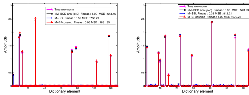
Figure 4: Examples of estimated row-norm using 3 different algorithms. left) M = 128 , N = 64 , k = 10 and L = 3 . right) M = 64 , N = 64 , k = 10 and L = 3 . Here, we want to illustrate cases where a “good” sparsity recovery does not necessary lead to low mean-square error.
