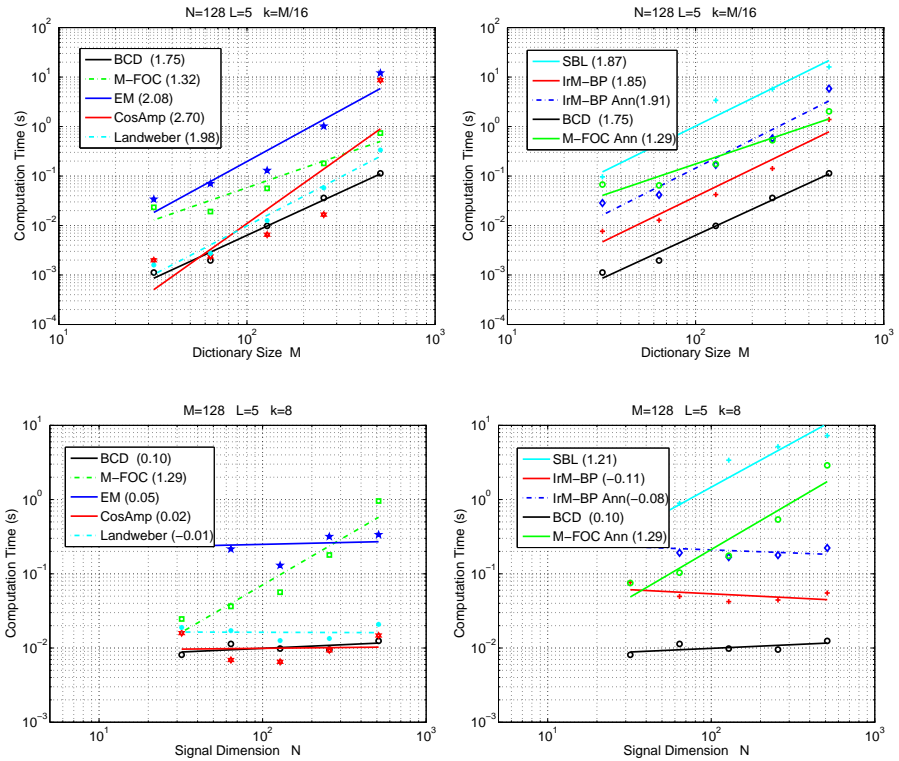
Figure 2: Estimating the empirical exponent, given in parenthesis, of the computational complexity of different algorithms (M-BCD, IrM-BP, M-SBL, M-FOCUSS, CosAmp, Landweber iterations). The top plots give the computation time of the algorithms with respects to the dictionary size. The bottom plots respectively depict the computational complexity with respects to the signal dimensionality. For a sake of readability, we have separated the algorithms in two groups :(left) the ones that solve \ell_1 - \ell_q problem. (right) the ones that solve \ell_p - \ell_2 problem (M-BCD result provided for baseline comparison). The “IrM-BP Ann” and “M-FOC Ann” refers to the Ir-MBP and M-FOCUSS algorithm using an annealing approach for iteratively decreasing \varepsilon as described in Algorithm (??).
