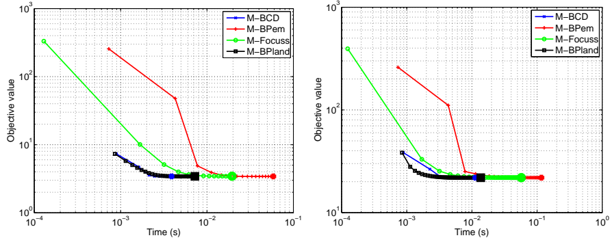
Figure 1: Examples of objective value evolution with respects to computational time. Here we have, M = 128 , N = 64 , L = 3 . The number of active elements is : left) k = 5 . right) k = 32 . For each curve, the large point corresponds to the objective value at convergence.
