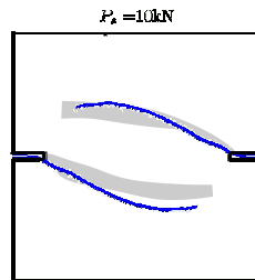
Figure 7: Comparison of experimental (gray zone) and simulated (thick line) crack paths for K_{Ic} = 1 \text{ MPa}\cdot\text{m}^{1/2} and a 10-kN shear preload.
