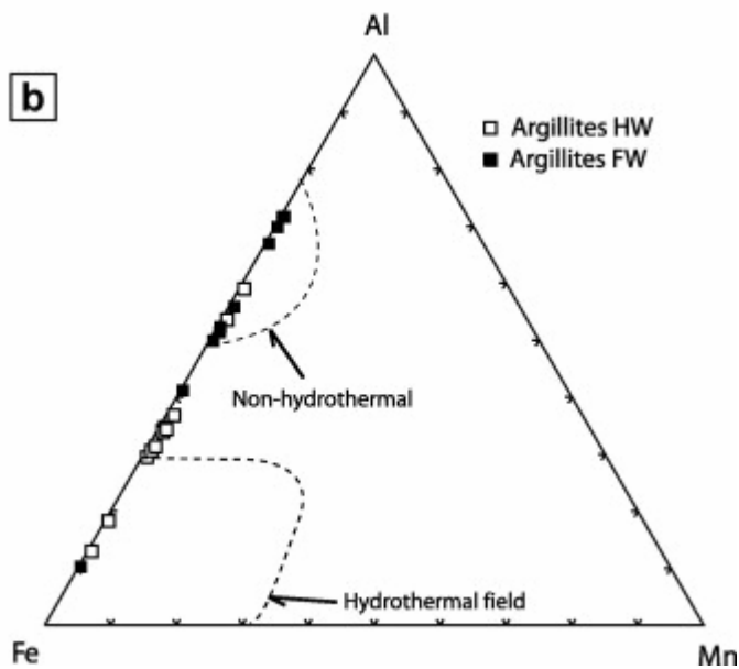
Fig. 5. : (a) Al/(Al + Fe + Mn) - (Fe/Ti) for Koudiat Aïcha argillites (after Boström, 1973 ), illustrating the pronounced terrigenous contribution to these rocks. (b) Al–Fe–Mn ternary plots for Koudiat Aïcha argillites (footwall and hanging wall), showing hydrothermal and non-hydrothermal field (after Boström, 1973 ; see text).
