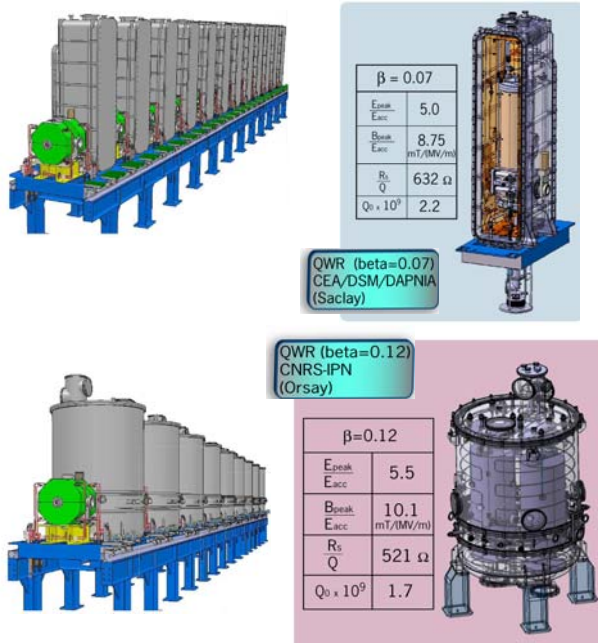
Figure 7: The SPIRAL2 superconducting cryomodules (top: \beta=0.07 , bottom: \beta=0.12 )
