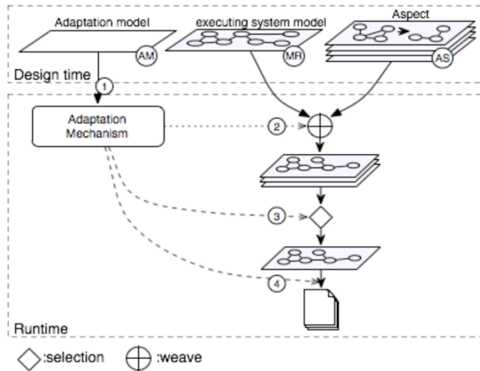
Fig. 1. Overall MDE/AOM approach for adaptive systems
