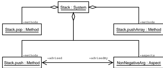
Figure 5: Object diagram of the impacted methods model of the stack example.
