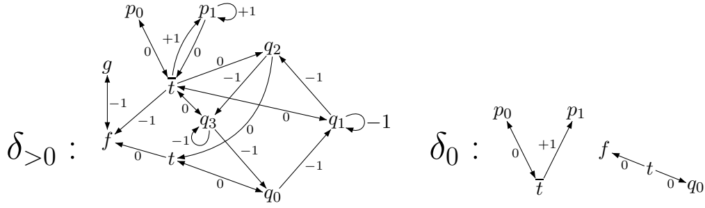
Figure 1: The one-counter net \mathbb{O} for which CTL model checking is PSPACE-hard
