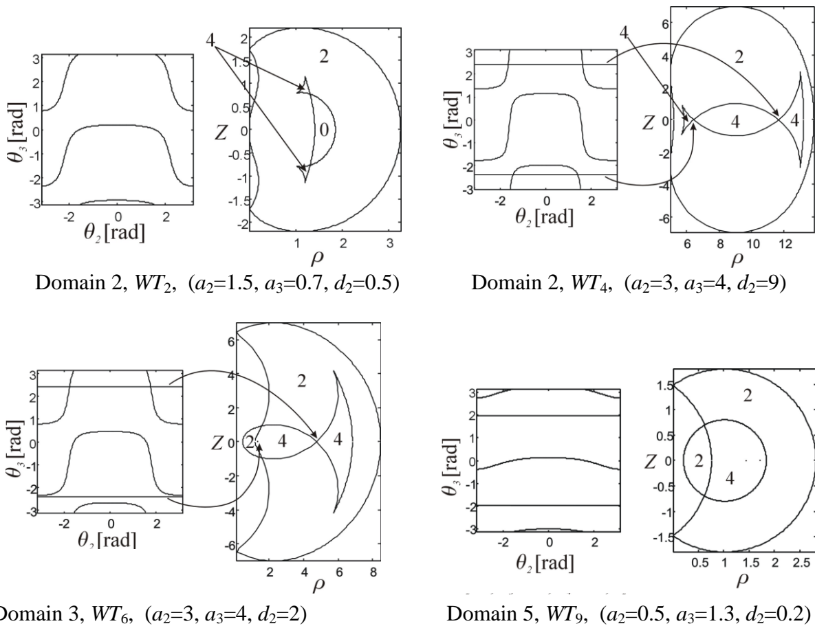
Fig. 13. Workspace topologies WT_2 , WT_4 , WT_6 and WT_9 .
