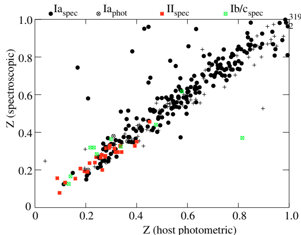
Fig. 4. SNLS spectroscopic redshifts vs. host photometric redshifts taken from the catalog of Ilbert et al. (2006). Spectroscopically identified supernovae and photometrically identified SNIa are marked by the signs defined at the top of the figure. The crosses are supernovae whose type is not determined spectroscopically or photometrically.
