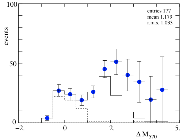
Fig. 11. The distribution of \Delta M_{570} . The solid histogram shows the distribution of \Delta M_{570} for events with m_{570} < 24.1 and 0.05 < z < 0.4 . The dashed histogram shows the distribution for spectroscopically and photometrically selected SNIa. The data points with error bars show the number of events after correction for the detection efficiency and the dependence of the survey volume on \Delta M_{570} .
