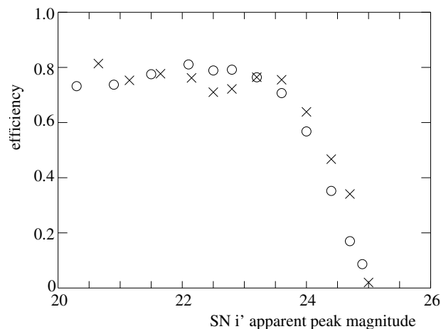
Fig. 5. Pre-selection efficiency as a function of i' . The “efficiency” is defined as the number of reconstructed events in a given magnitude interval divided by the number of generated events in the same interval. The circles are for SNIa and the crosses for SNcc with \tau_{\text{fall}} = 100 days.
