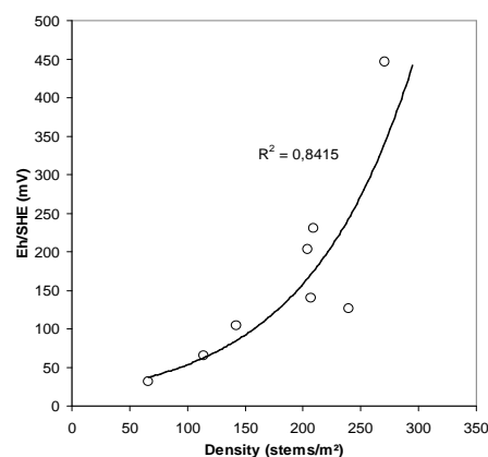
Figure 7: Correlation between reed density and redox potential of the sludge deposits for pilots fed with septage with a compost filtration layer and during the
