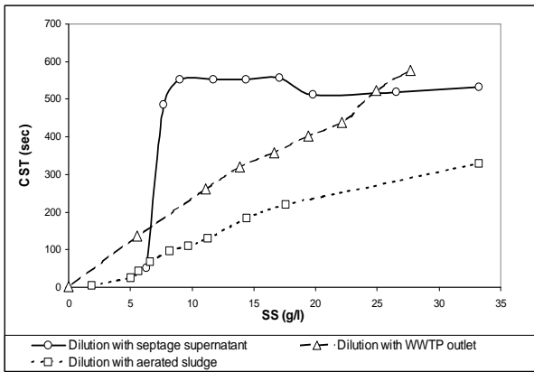
Figure 1: Sludge dewaterability (CST) at different suspended solids concentration obtained with septage supernatant, WWTP outlet, or with aerated sludge dilutions.
