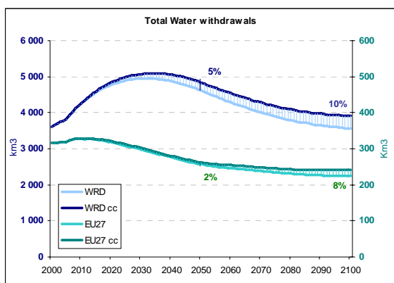
Figure 5 : World and EU27 total water withdrawal with and without climate change up to 2100
