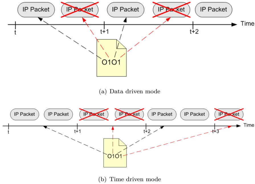
Figure 10: KauNet loss insertion
