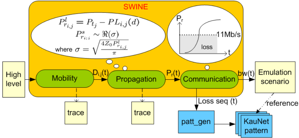
Figure 3: SWINE Architecture
