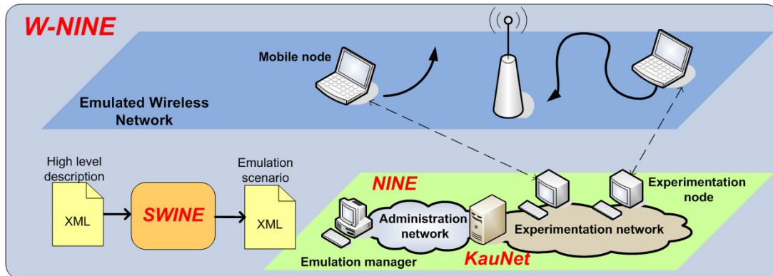
Figure 2: W-NINE Architecture.
