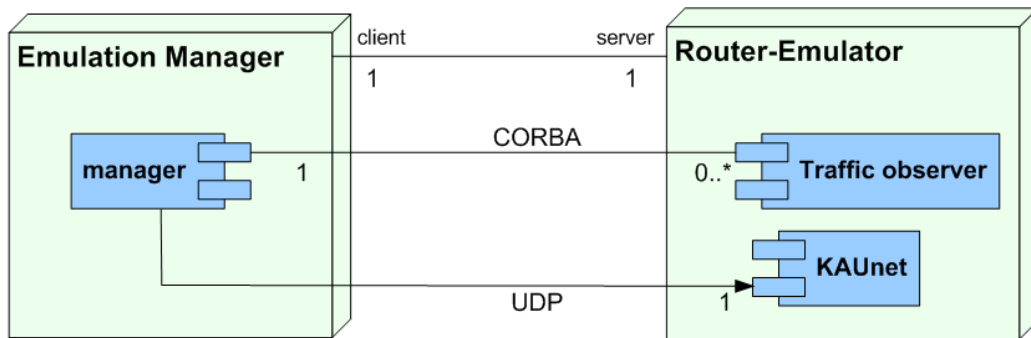
Figure 11: W-NINE deployment diagram
