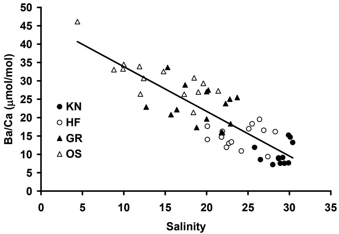
Figure 6. Salinity versus [Ba/Ca]_{water} , including data from all sites and sampling dates, with the linear relationship [Ba/Ca]_{water} = -1.22 (\pm 0.21) * Salinity + 46.05 (\pm 4.57) ( R^2 = 0.73 , n = 55 , p < 0.0001 ). See Fig. 1 for site abbreviations.
