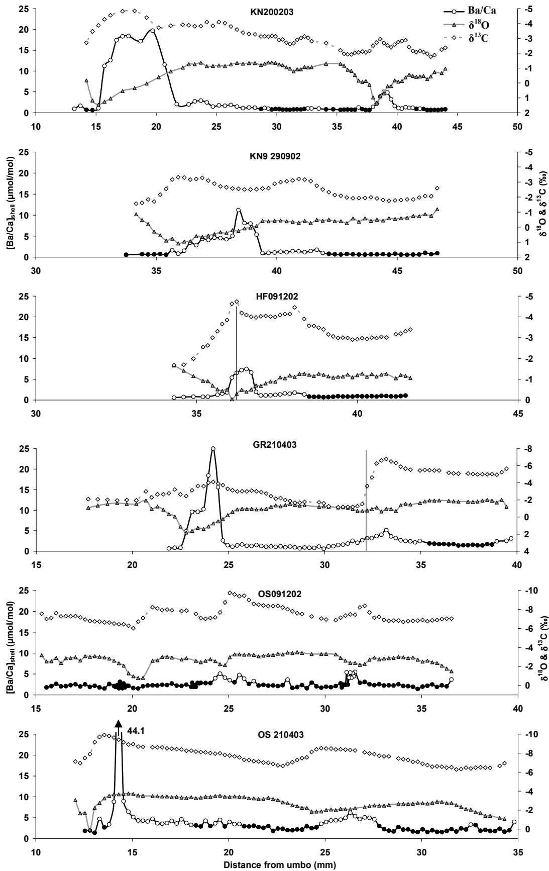
Figure 7. High resolution \delta^{18}\text{O} , \delta^{13}\text{C} , and [Ba/Ca]_{shell} profiles from the six shells. Black filled symbols denote data selected as background [Ba/Ca]_{shell} data. Vertical lines correspond to the time of transplantation (HF and GR shells only, see Materials and methods) as determined from the calcein stain. Shell codes represent collection site and date (format: ddmmyy). Note that the isotope axes are inverted.
