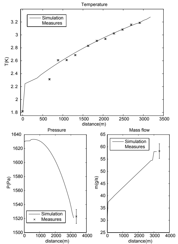
Figure 5: Temperatures, pressures and mass-flows along the header B in steady-state compared with experimental measurements
