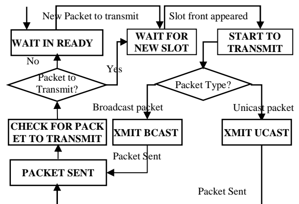
Figure 5: Slotted-TH illustration
