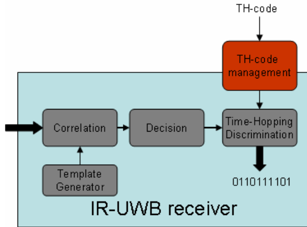
Figure 7. Implementation of TH-code reconfiguration in TH-BPAM receiver.
