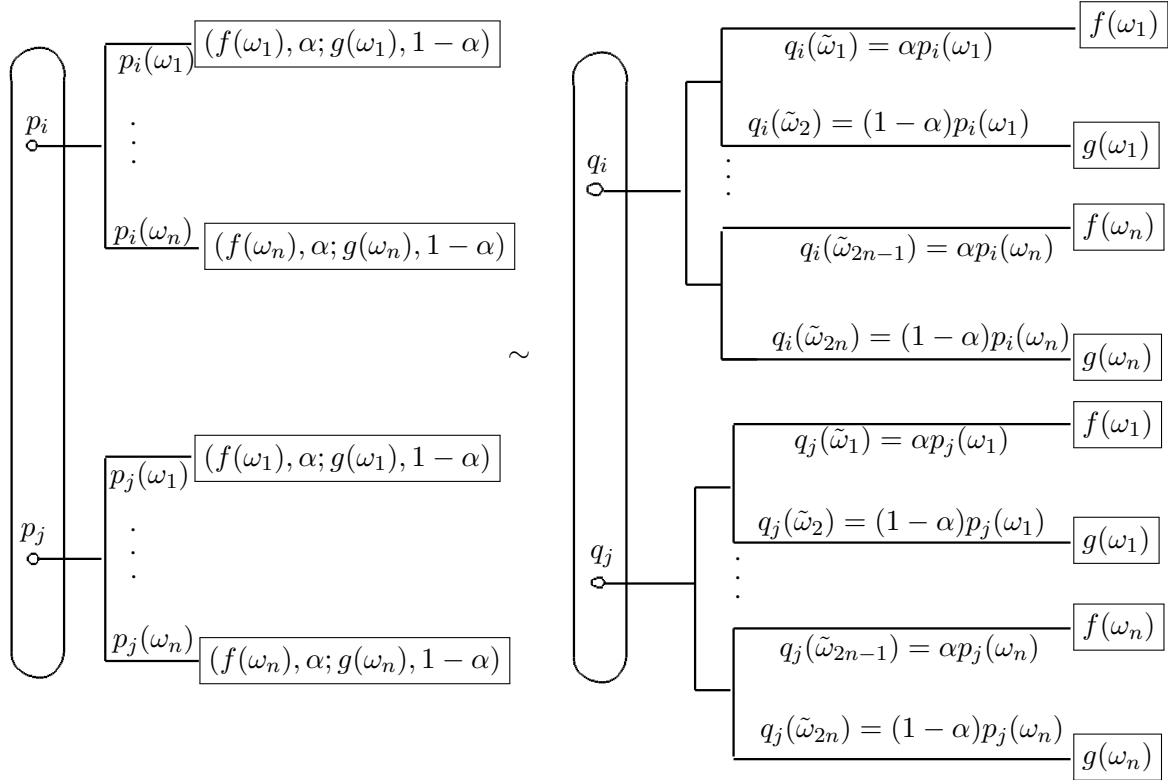
Figure 1: Decomposition Indifference
