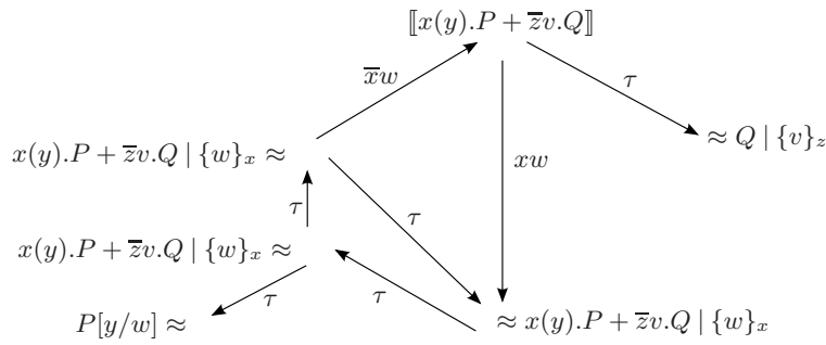
Fig. 2. Transitions of the \pi_\alpha encoding of the \pi_B sum in Figure 1.
