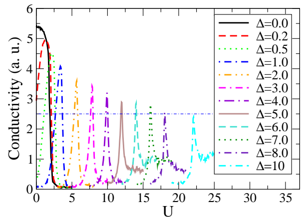
FIG. 8: (Color online). Conductivity for low and high values of U and different values of \Delta . ( t = 1, kT = 0.01 ).
