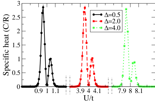
FIG. 2: (Color online). The molar specific heat at kT = 0.01 for different values of \Delta .
