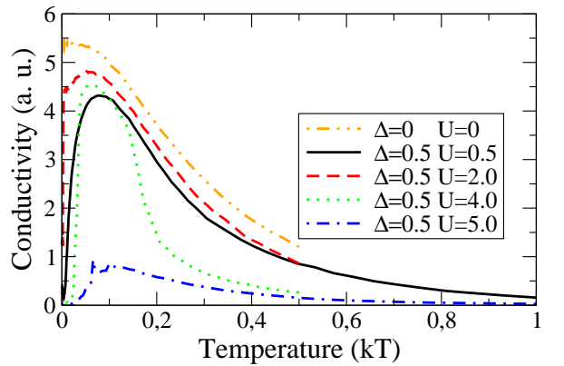
FIG. 13: (Color online). Conductivity curves at high temperatures for \Delta = 0.5 and different values of the coulombian repulsion U .
