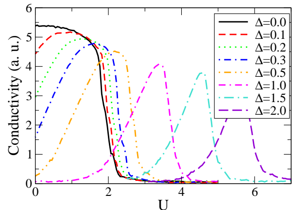
FIG. 9: (Color online). DC Conductivity for low values of U and different values of \Delta . ( t = 1, kT = 0.01 ).
