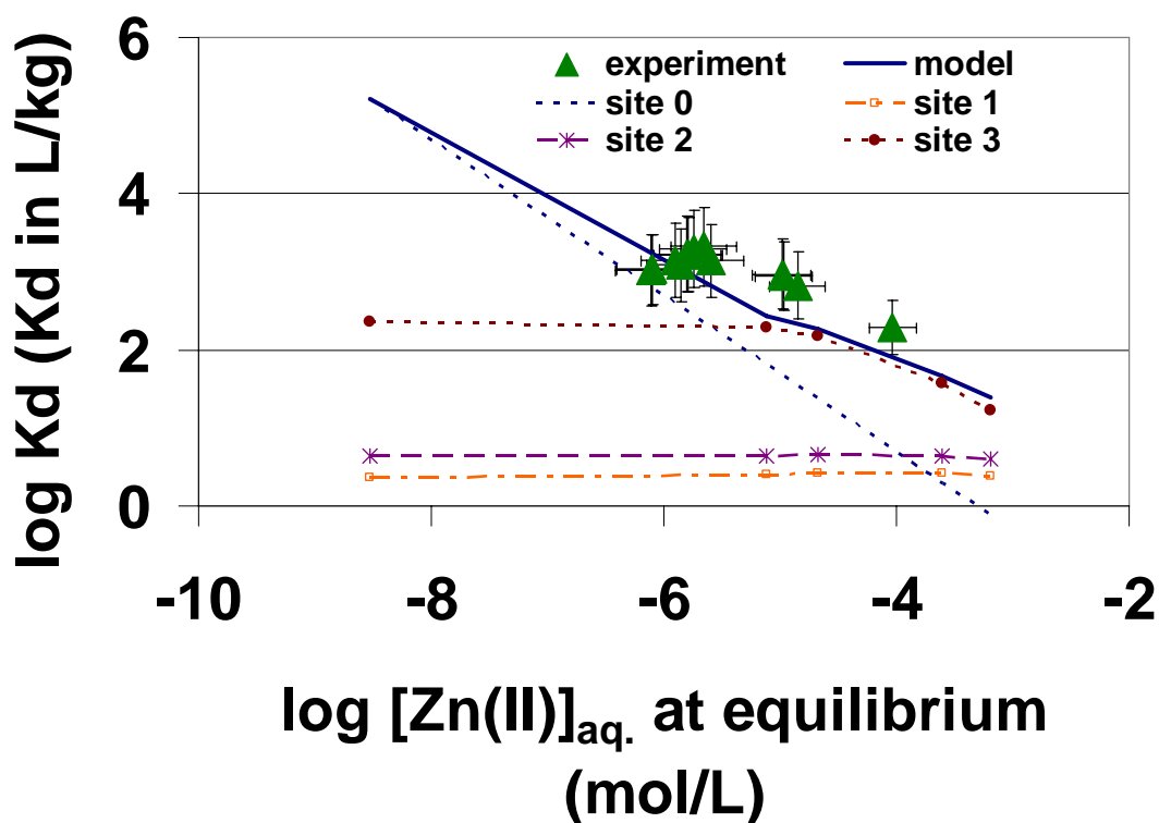
Figure 9: Comparison between measured (symbols) and predicted (continuous lines) Kd data for Zn(II), as a function of the aqueous zinc concentration. Case of isotherms obtained with the “Auby” sediment in (A) 10 -2 M NaCl (pH=7.8±0.1) and (B) 10 -2 M CaSO 4 (pH=7.6±0.1). Both graphs show the contribution of each site to the predicted sorption curve.
