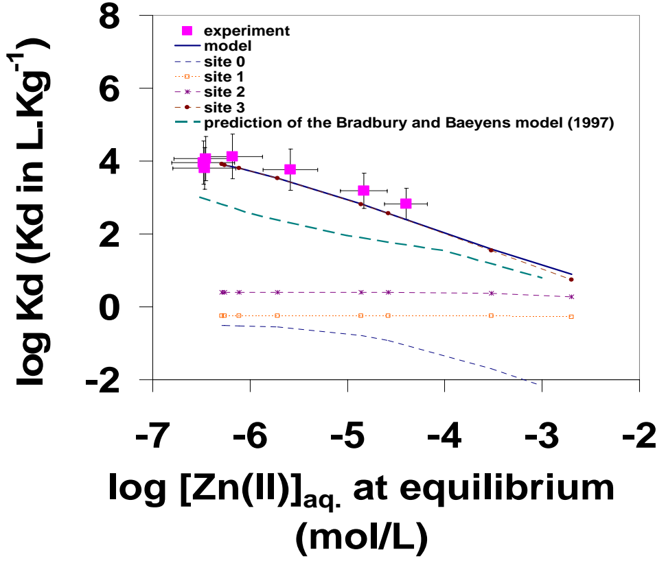
Figure 7: Comparison between measured (symbols) and predicted (continuous lines) Kd data for Zn(II), as a function of the aqueous zinc concentration. Case of isotherms obtained for the “Pech Rouge” soil in (A) 10 -2 M NaCl (pH=7.9±0.1) and (B) 0.5 M NaCl (pH=8.5±0.1) Both graphs show the contribution of each site to the predicted sorption curve. On Figure B, the prediction of the data by using the Bradbury and Baeyens (1997) model is shown.
