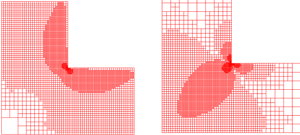
Figure 5. Adaptive meshes as obtained by a refinement criteria based on the Kelly error estimator: (left) for the temperature u ; (right) for the potential \phi .
