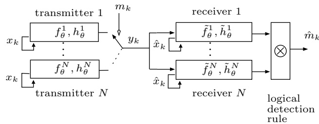
FIG. 2.4 – Chaotic switching
