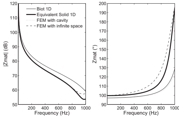
FIG. 8. Simulation of the mechanical impedance of foam A: L=20 mm, E= 280 kPa, \eta=0.17 , \nu=0 .
