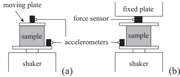
FIG. 1. Classical measurement set-up: (a) seismic test; measurement of the ratio of the velocities between the shaker table and the top mass, (b) compression test; measurement of the ratio of the force transmitted by the porous sample to the fixed plate F on the velocity of the shaker table v .
