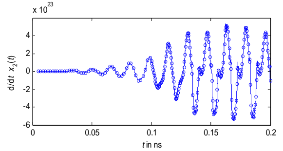
Fig. 4. Solid line: given training data. Marker "o": Output of trained ANN with ten neurons.
