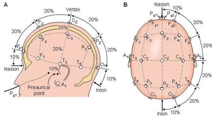
Fig. 1. 10-20 system
