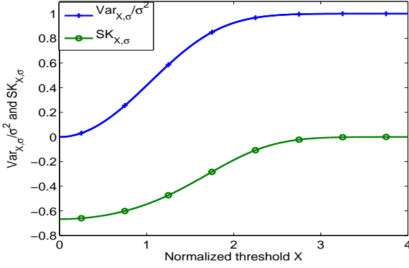
Fig. 1. Evolution of the normalized variance and the spectral kurtosis in function of the normalized threshold X_n = \frac{X}{\sigma} .
