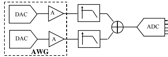
Figure 3: Experimental setup
