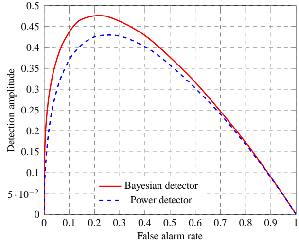
Fig. 1. Detection amplitude comparison in SIMO - M = 1, N = 8, L = 20, \text{SNR} = -10 \text{ dB}
