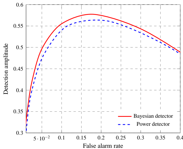
Fig. 2. Detection amplitude comparison in MIMO - M = 2, N = 8, L = 10, \text{SNR} = -10 \text{ dB}
